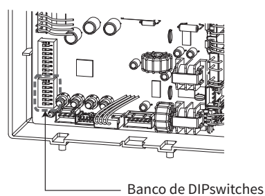
Modelos TKGU-38-IN y TKGU-38-EN
